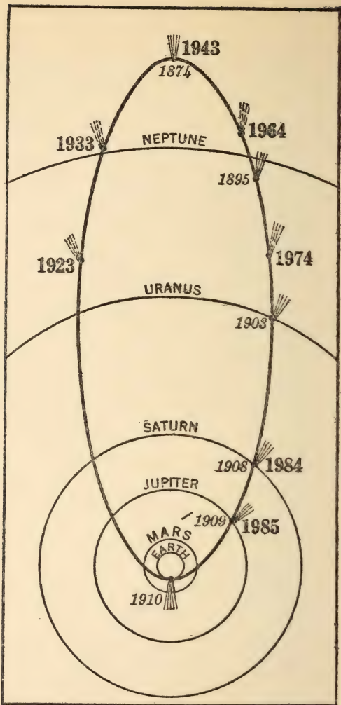
The orbit of Halley's Comet, which it passes over in 75 to 77 years, showing where the comet is to be found now, and during its course until its next return in 1985.
